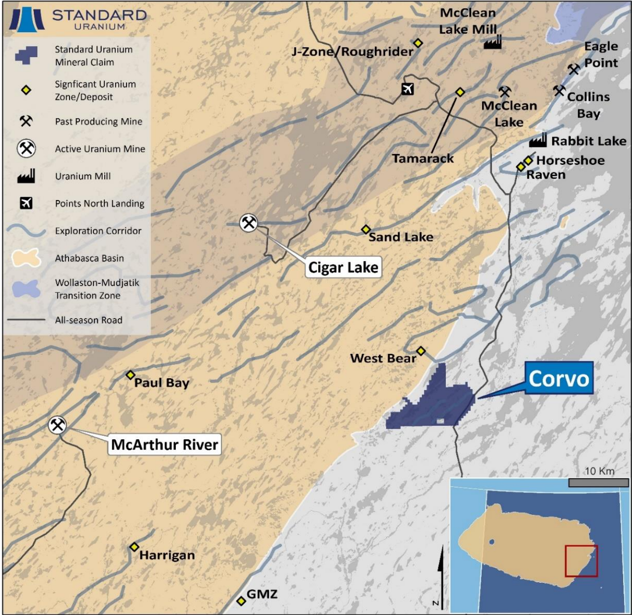
Figure 1. Overview map of Standard Uranium's Corvo Project. The newly expanded Corvo Project is located 45 km northeast of the 92Energy's Gemini Mineralized Zone ("GMZ") and 60 km due east of Cameco's McArthur River mine.
