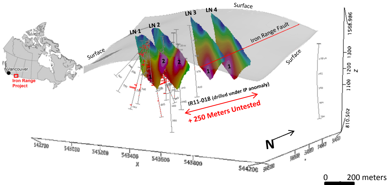
Figure 1. Talon Zone 2011 Surface IP Inversion Models (chargeability) oriented in 3D (looking northwest) along with drill holes showing gold intercepts + 0.5 gpt Au (red bar plots). Anomaly 1 is continuous across all 4 IP lines and is spatially associated with mineralization on lines 1 and 2. Anomaly 2 is present on lines 1 and 2. Lines 3 and 4 did not extend far enough south to detect anomaly 2.
